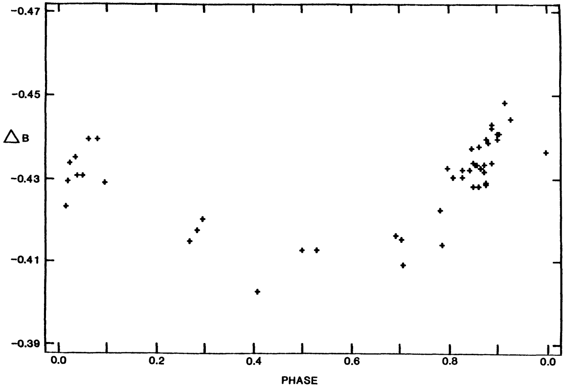
Figure 1. Photoelectric B band observations of HR 1063 relative to HR 1051, phased together with a period of 2.49246 days.
