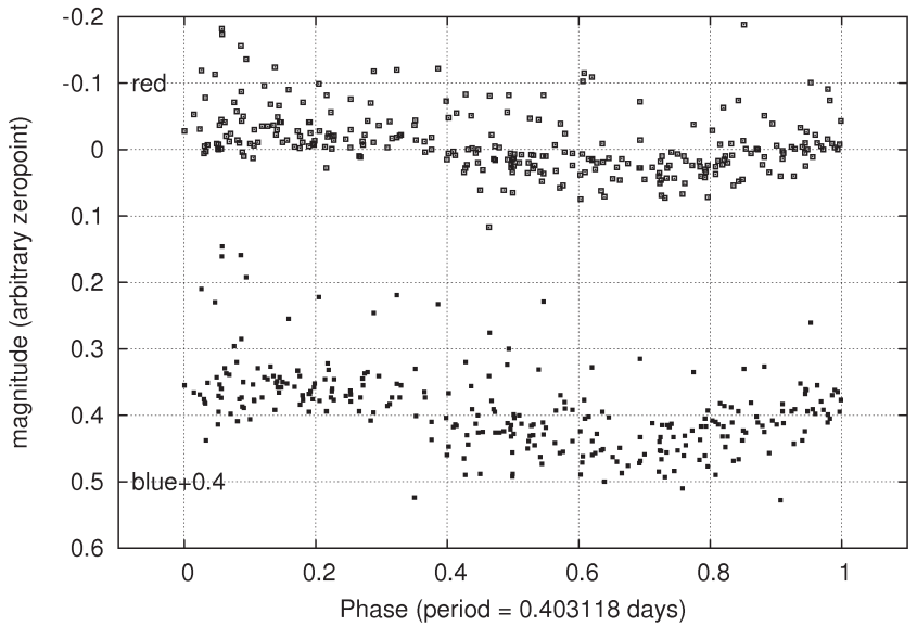
Figure 12. Phased light curve of residuals of star 125.23719.00262.
