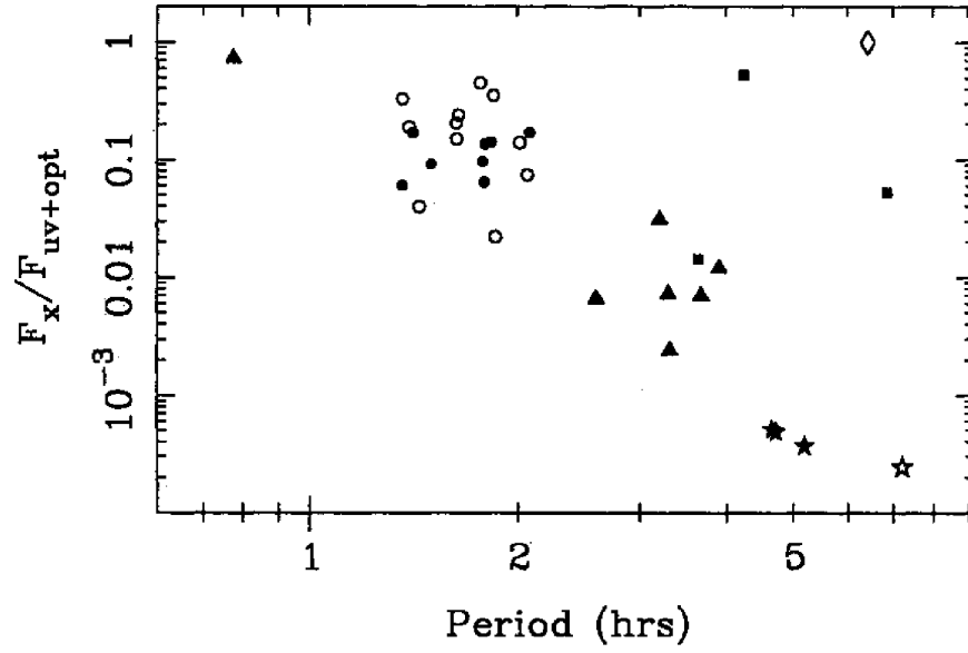
Figure 1. Flux ratio versus orbital period for CVs.
