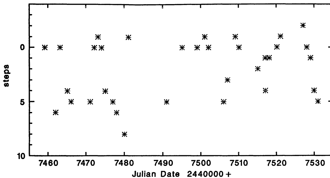
Figure 1. The light curve of \pi PsA from JD 24475455 through 24475532. Points indicate visual estimates by the author (Argelander steps). The comparison stars are SAO 214615 ( \beta Scl); SAO 191550; and SAO 191581.
